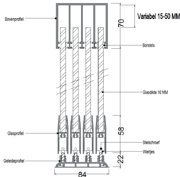
4 Spoor Glaswand
