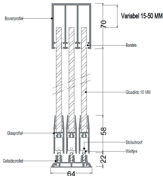
3 Spoor Glaswand
