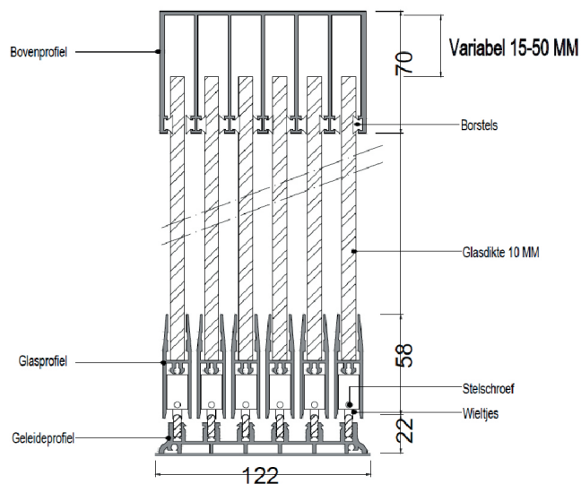
6 Spoor Glaswand
