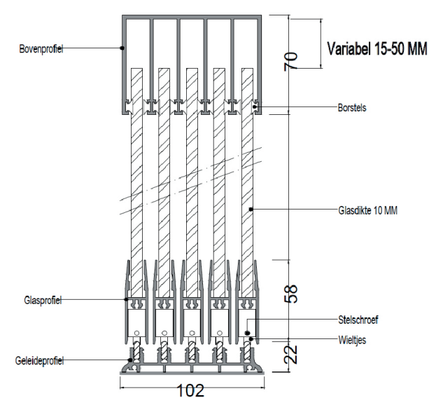
5 Spoor Glaswand
